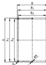
BAK 30-70 (见上表) 铜: 30-70 铝: 30-70
